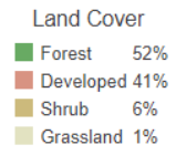
Slope Angle (top), Land Cover (middle), Tree Cover (bottom)
