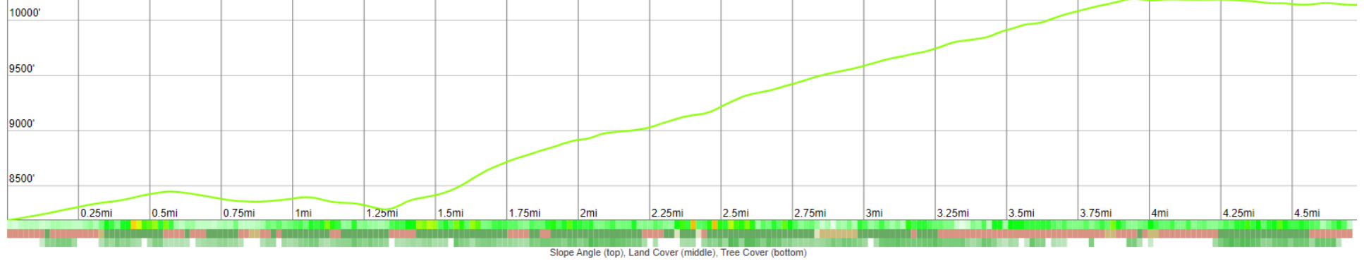
Slope Angle (top), Land Cover (middle), Tree Cover (bottom)
